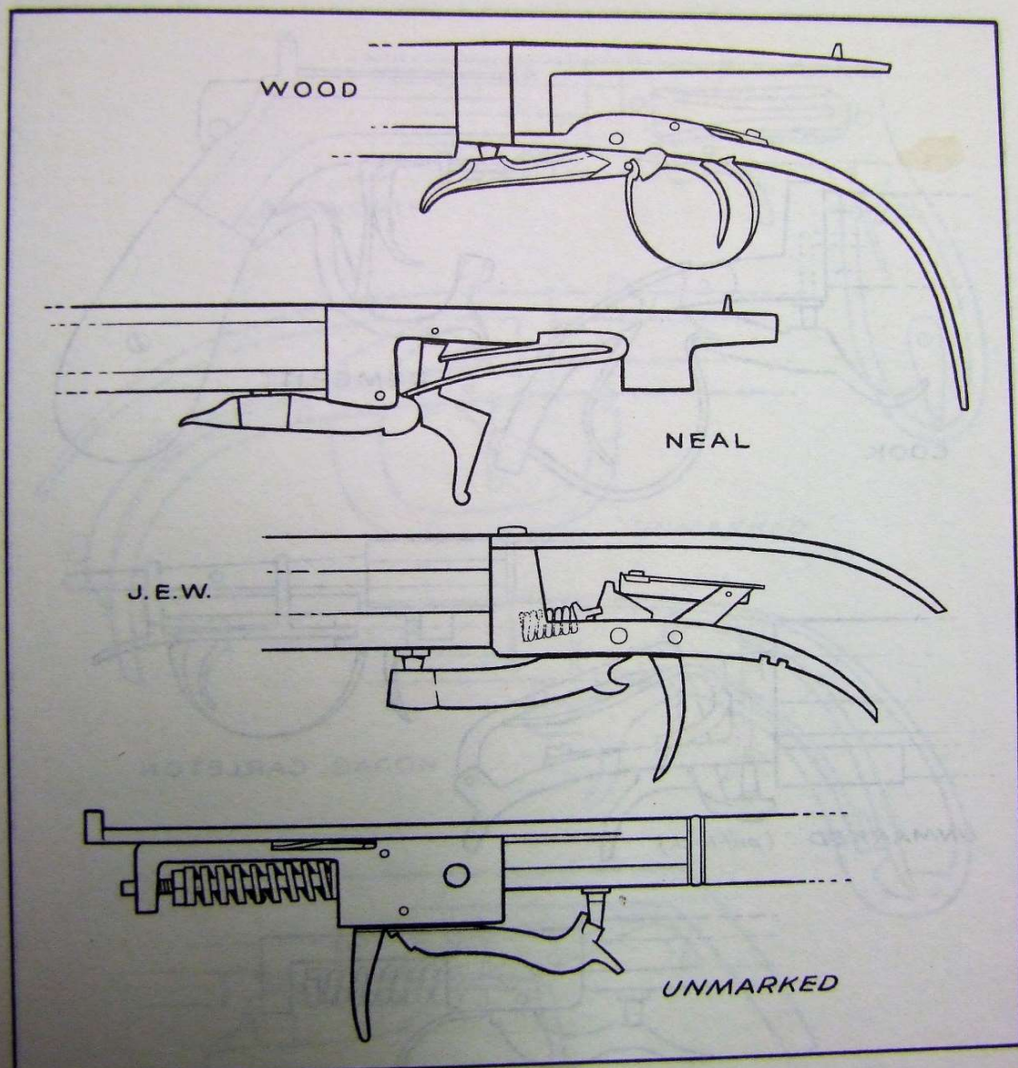
FIGURE 17. Owing to the simple mechanism to be found on the vast majority of Underhammers, it is felt that the cross-sections to be seen in this figure and in figures 18, 19, and 20 require no further explanation.
